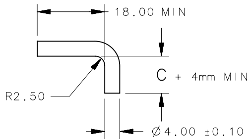
RECOMMENDED L FITTING DIMENSIONS FOR ROD OR CABLE ACTUATED APPLICATIONS SCALE 1:1
