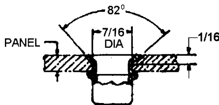
INSTALLATION METHOD "A"
